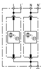
Basic circuit diagram DV M TN 255
